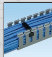
For Type G and H Wiring WR2-C – for 2" duct width WR3-C – for 3" duct width WR4-C – for 4" duct width WR5-C – for 5" duct width WR2H-C – for 2" hinged duct
