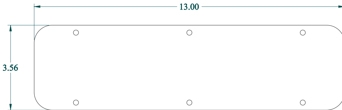
FRONT VIEW
