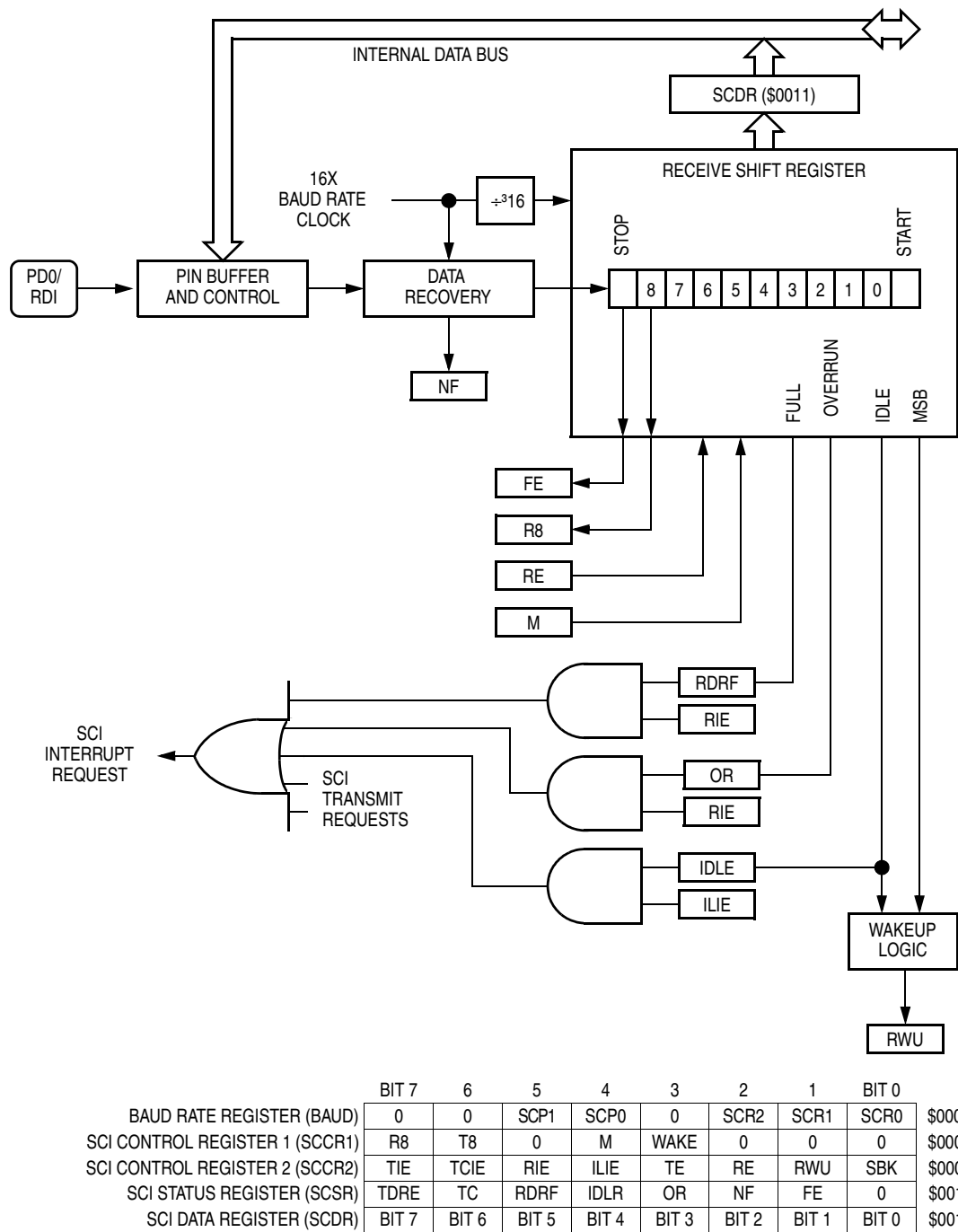
Figure 9-3. SCI Receiver
