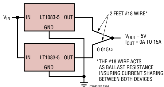
Paralleling Regulators
