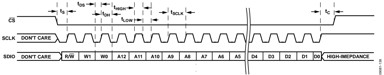
Figure 38. Serial Control Port Read—MSB First, 16-Bit Instruction, One Byte of Data
