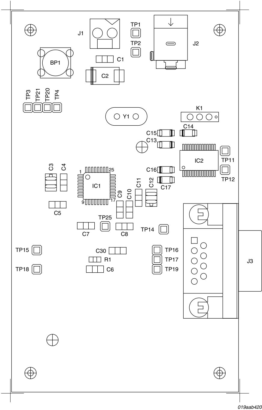
Fig 30. Design example - Components top view
