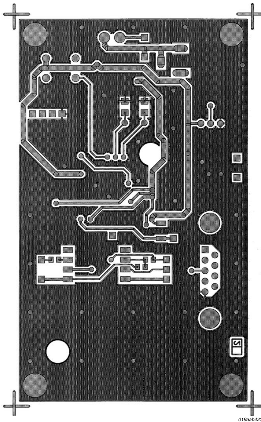
Fig 33. Design example – Layout bottom view
