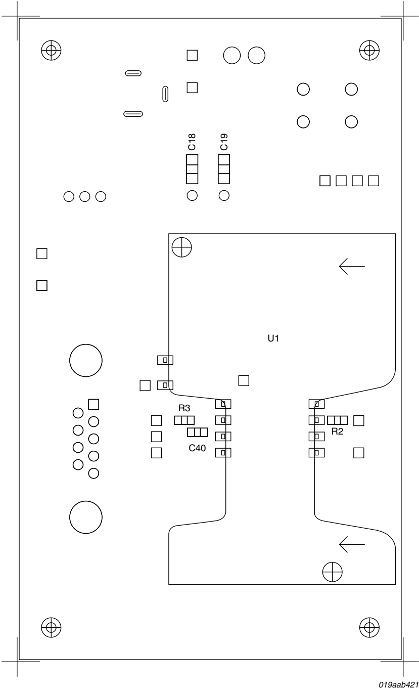
Fig 31. Design example - Components bottom view
