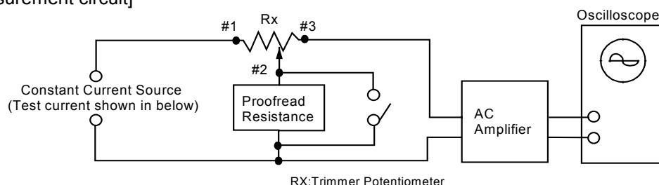
[Measurement circuit]
