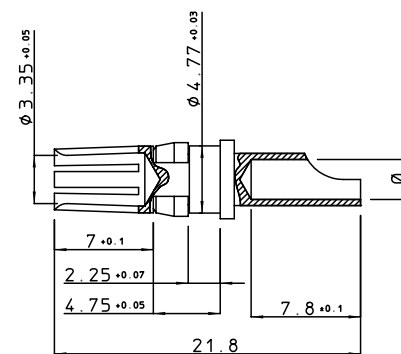
socket contact
