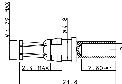
socket contact
