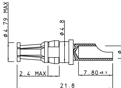
socket contact
