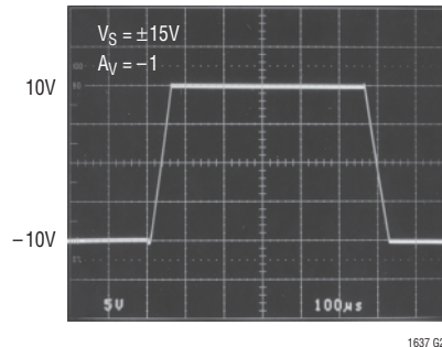
Large-Signal Response
