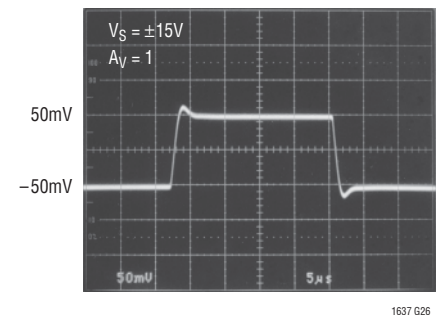
Small-Signal Response
