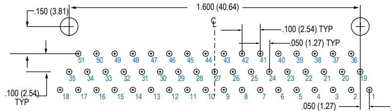
51 PIN
