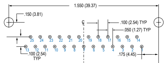
25 PIN
