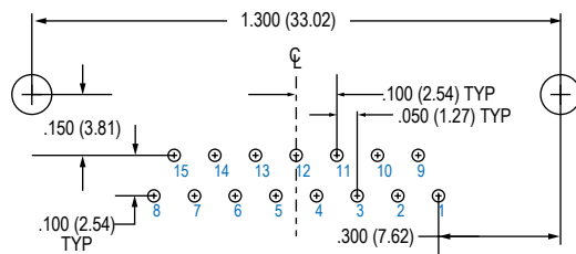
15 PIN
