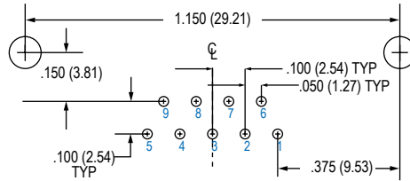
9 PIN
