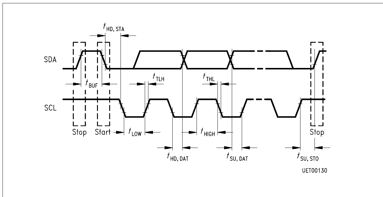
Figure 3 I²C-Bus Timing
