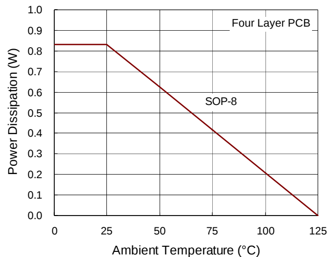
Figure 3. Derating Curves for RT8270 Packages
