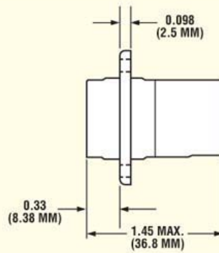
ECF Side View
