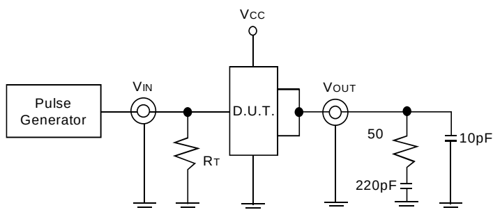
Figure 2. Z_o = 50\Omega AC Termination, C_L = 10\text{pF} The capacitor value for ac termination is determined by the operating frequency. For very low frequencies a higher capacitor value should be selected.
