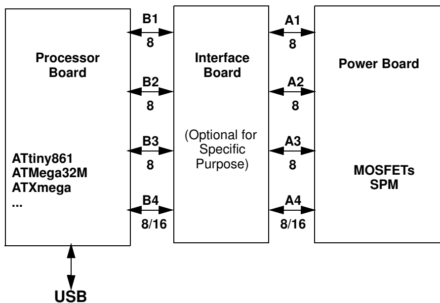
Figure 1-1. System Architecture
