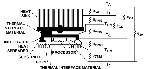
Figure 68. Thermal Model
