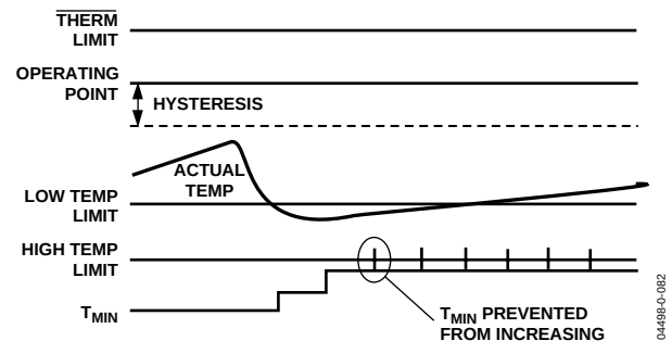
Figure 76. T_{MIN} Adjustments Limited by the High Temperature Limit
