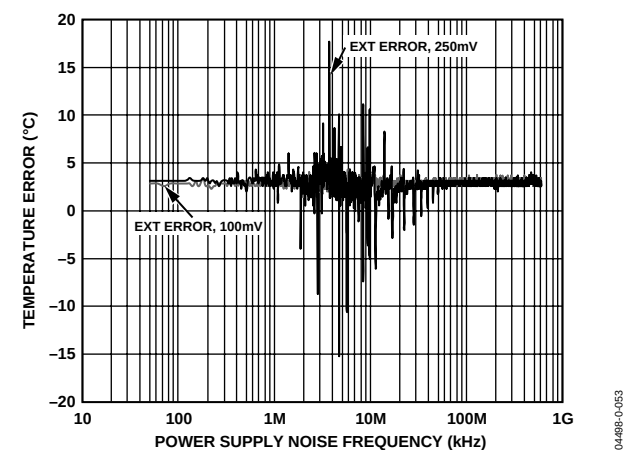
Figure 12. Remote Temperature Error vs. Power Supply Noise Frequency
