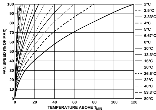
Figure 62. T RANGE vs. Actual Fan Speed Profile
