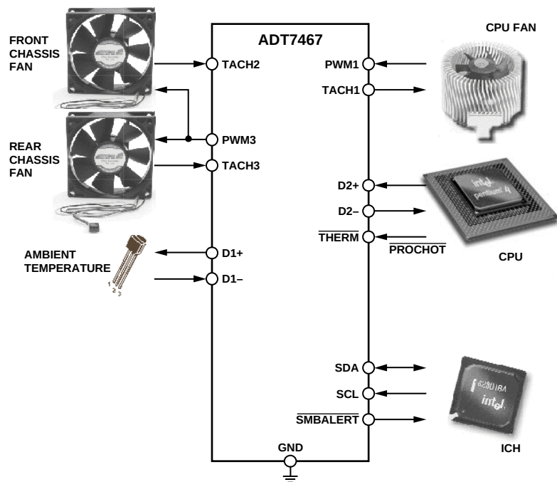
Figure 15. ADT7467 Configuration
