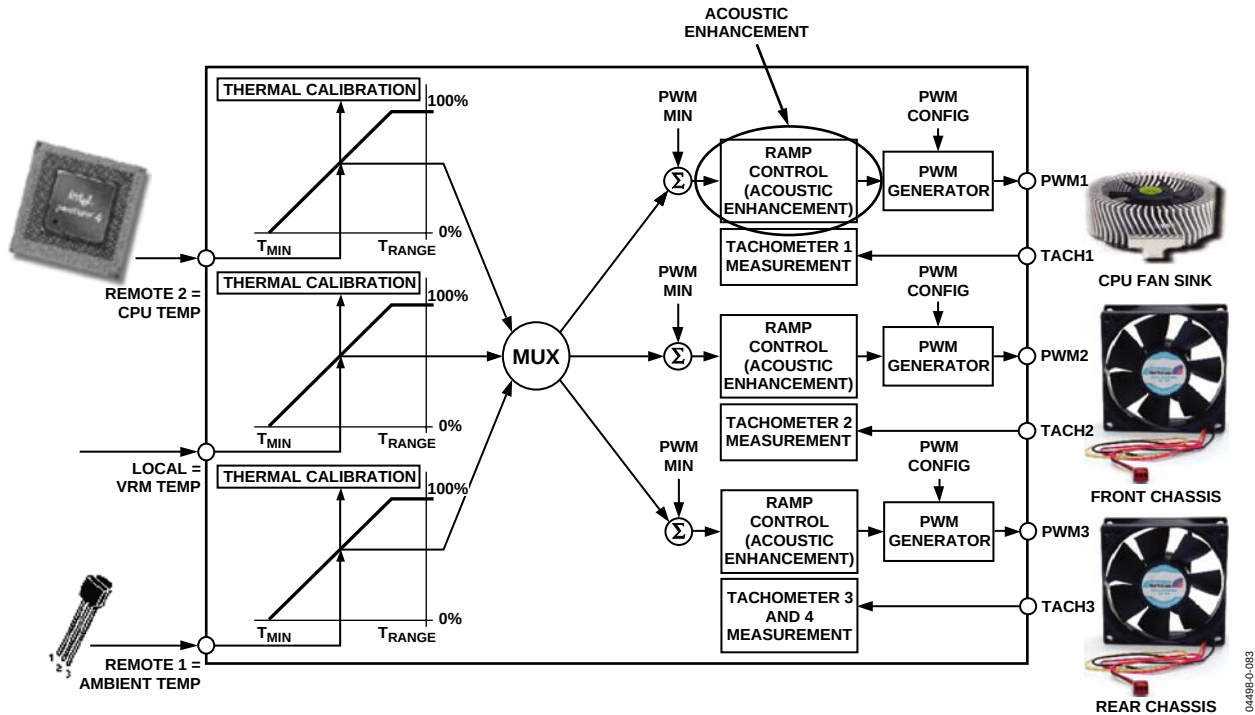
Figure 77. Acoustic Enhancement Smoothes Fan Speed Variations under Automatic Fan Speed Control
