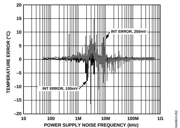
Figure 11. Internal Temperature Error vs. Power Supply
