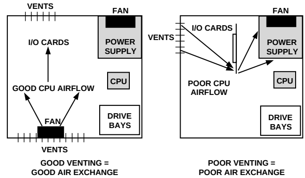
Figure 67. Chassis Airflow Issues
