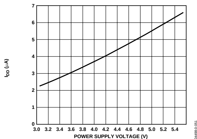
Figure 10. Shutdown I_{DD} vs. Power Supply
