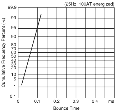
(2) Bounce Time
