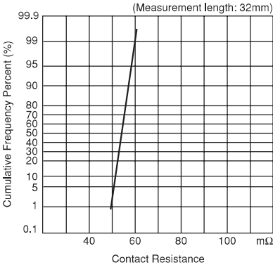
(2) Contact Resistance
