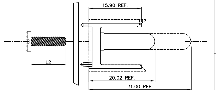
SINGLE GUIDE PIN ASSEMBLY
