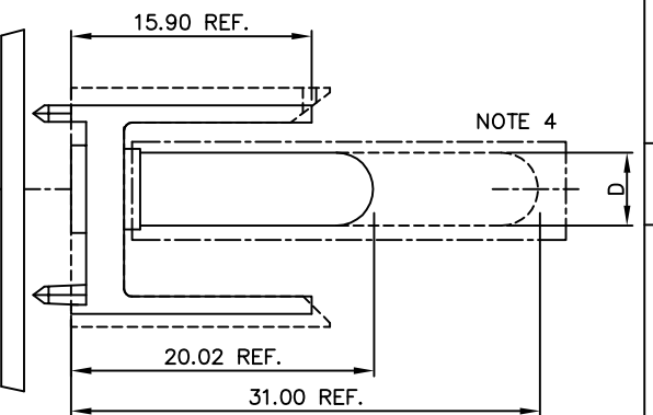
DOUBLE GUIDE PIN ASSEMBLY
