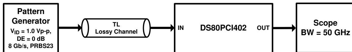
Figure 9-1. Test Setup Connections Diagram
