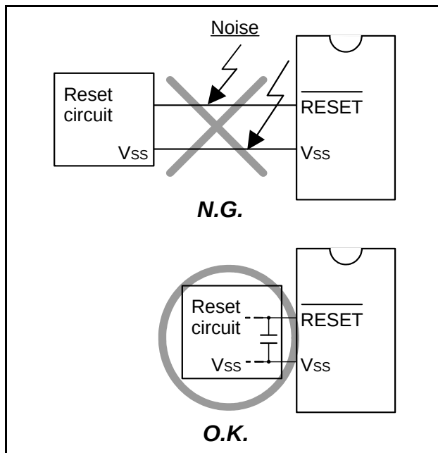
Fig 72. Wiring for the \overline{\text{RESET}} input pin
