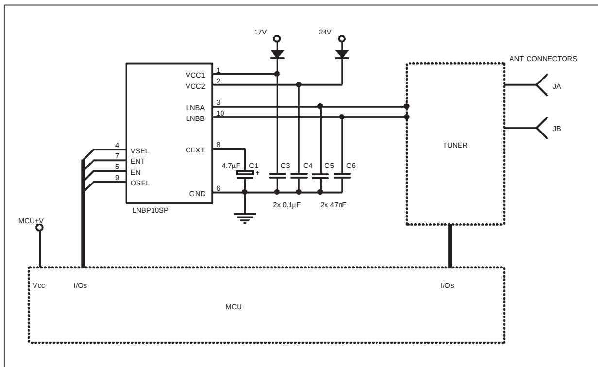
TWO ANTENNA PORTS RECEIVER: LOW COST SOLUTION
