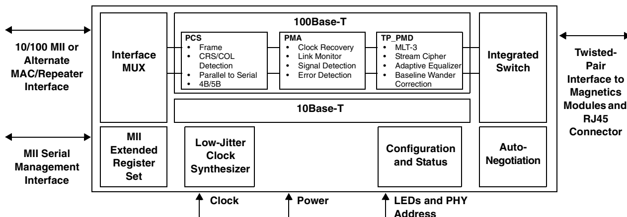
ICS1893BY-10 Block Diagram
