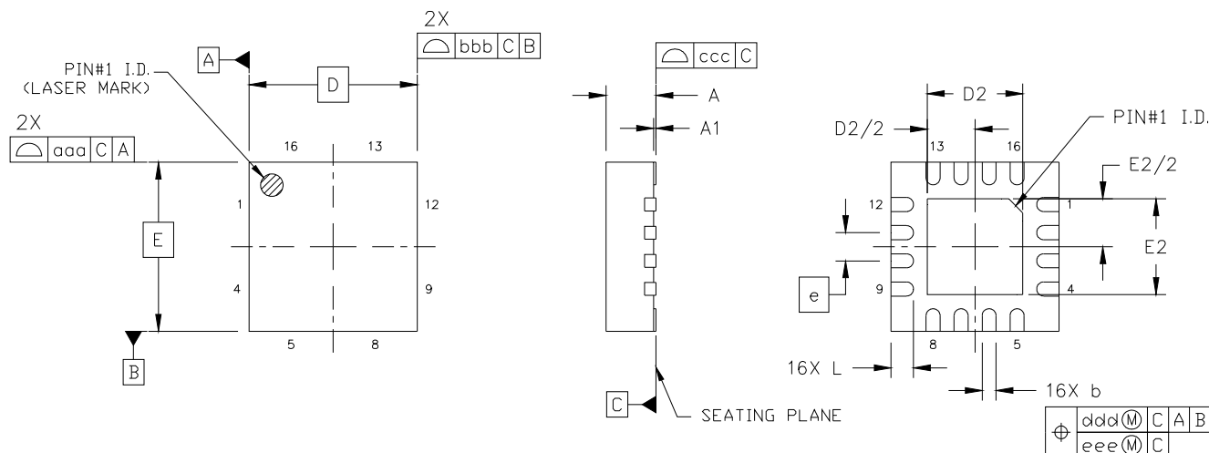
Figure 11. Si53323 3x3 mm 16-QFN Package Diagram
