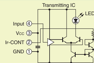
Transmitting module
