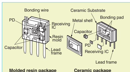
Internal structures of TOSLINK devices
