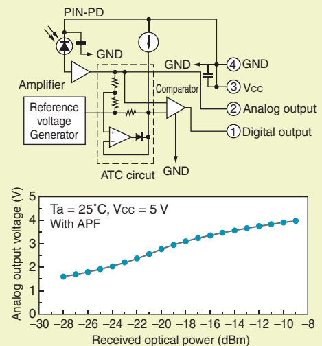
Receiving module with an analog output for optical flux monitoring
