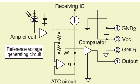
Receiving module
