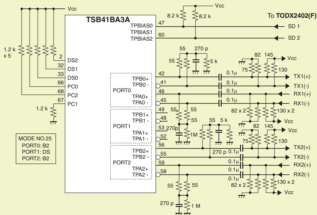
Connecting the TODX2402(F) to an IEEE 1394 PHY Layer IC
