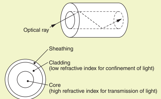
Structure of an optical fiber
