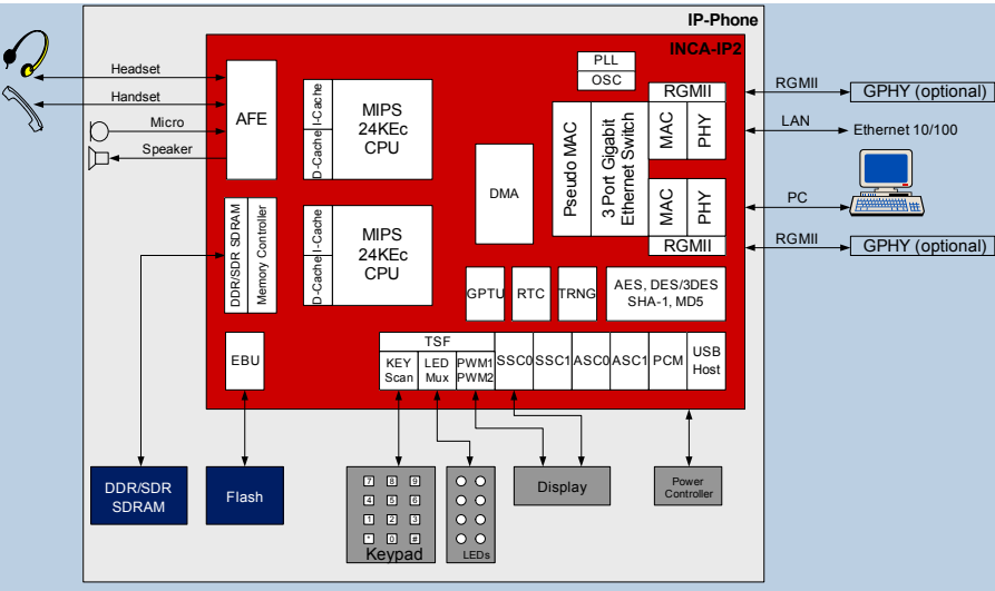
INCA - IP2 Block Diagram
