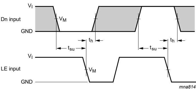
Measurement points are given in Table 8 . The shaded areas indicate when the input is permitted to change for predictable output performance. V_{OL} and V_{OH} are typical output voltage levels that occur with the output load.
