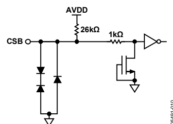
Figure 8. Equivalent CSB Input Circuit
