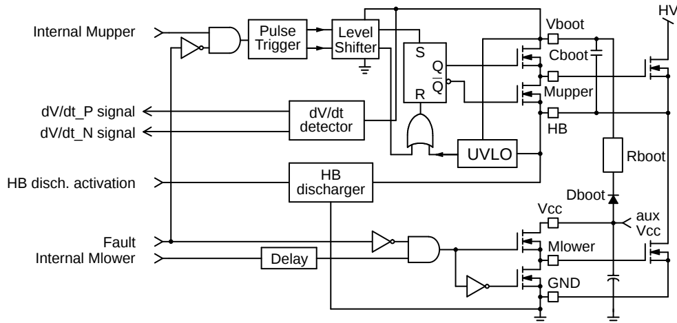
Figure 59. The NCP1399 Internal DRV's Structure
