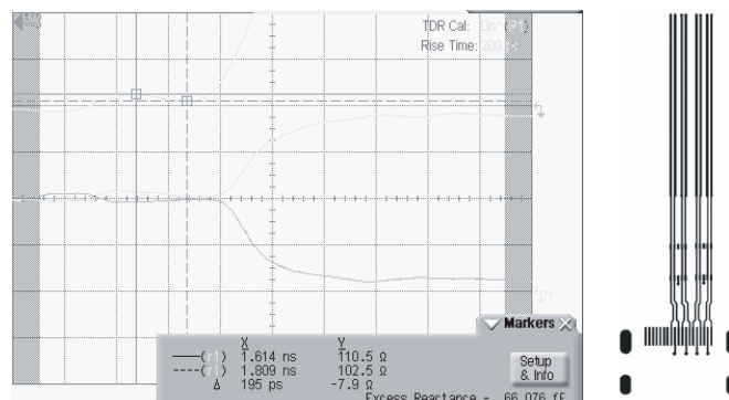
Figure 7. 120\Omega Differential Impedance Max 110\Omega , Min 102\Omega
