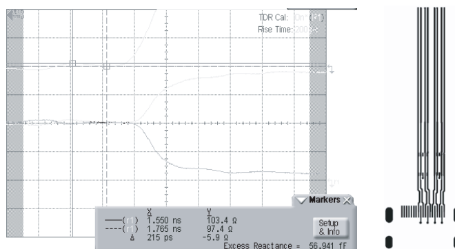
Figure 6. 100\Omega Differential Impedance Max 103\Omega , Min 97\Omega
