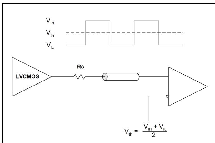
Figure 1A. DC-Coupling a Single LVCMOS Input to the IDT8SLVP1102
