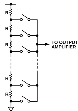
Figure 39. Resistor String
