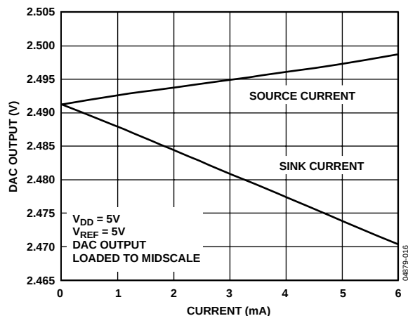
Figure 16. DAC V_{OUT} Source and Sink Current Capability
