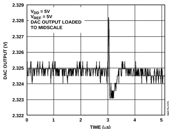
Figure 25. DAC-to-DAC Crosstalk
