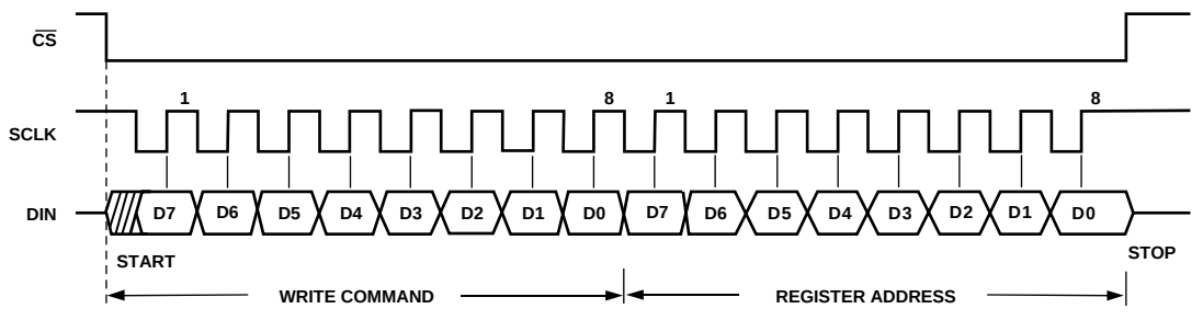
Figure 60. SPI—Writing to the Address Pointer Register to Select a Register for a Subsequent Read Operation
