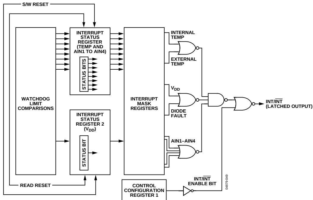
Figure 49. Interrupt Structure
