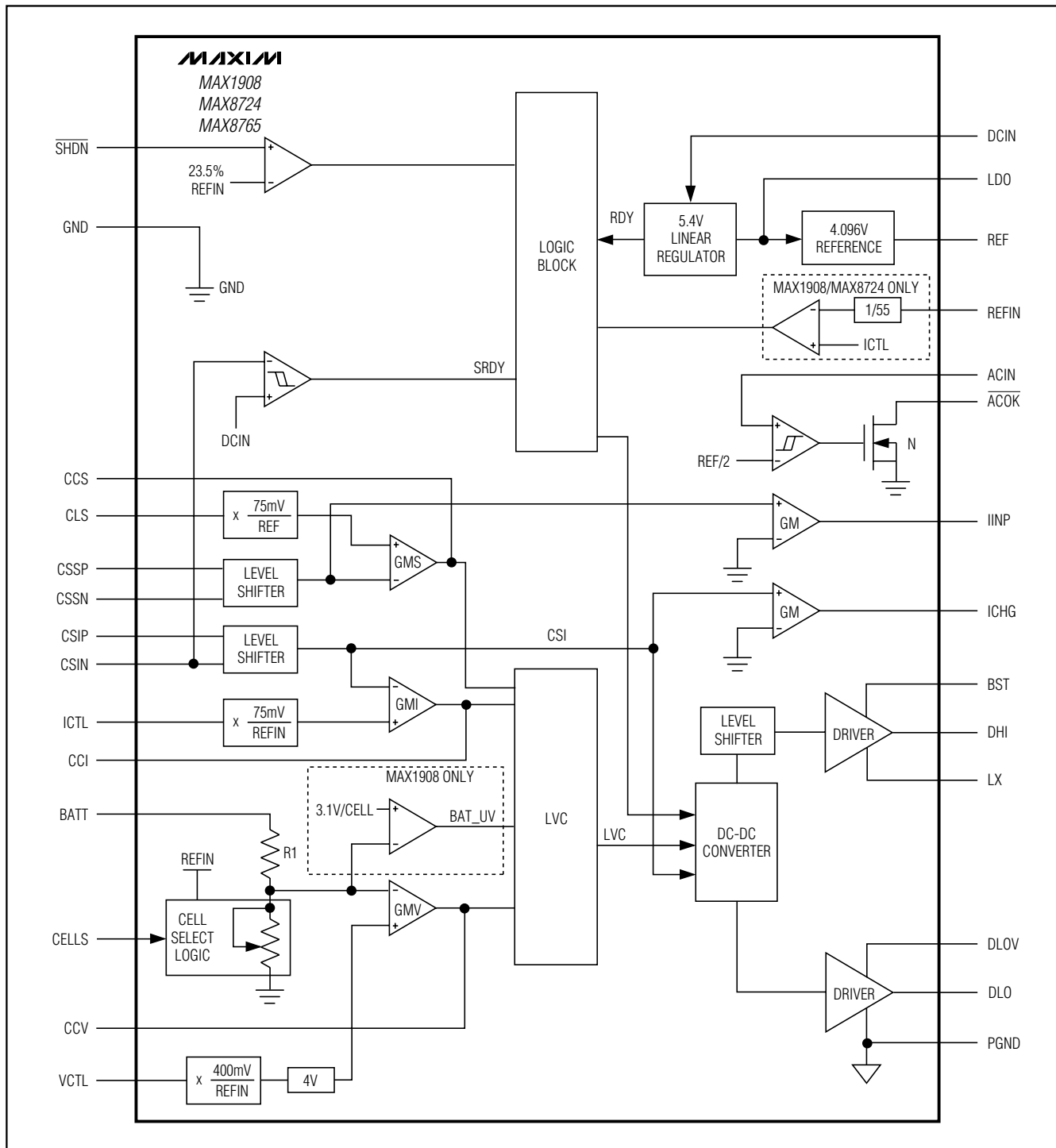
Figure 3. Functional Diagram
