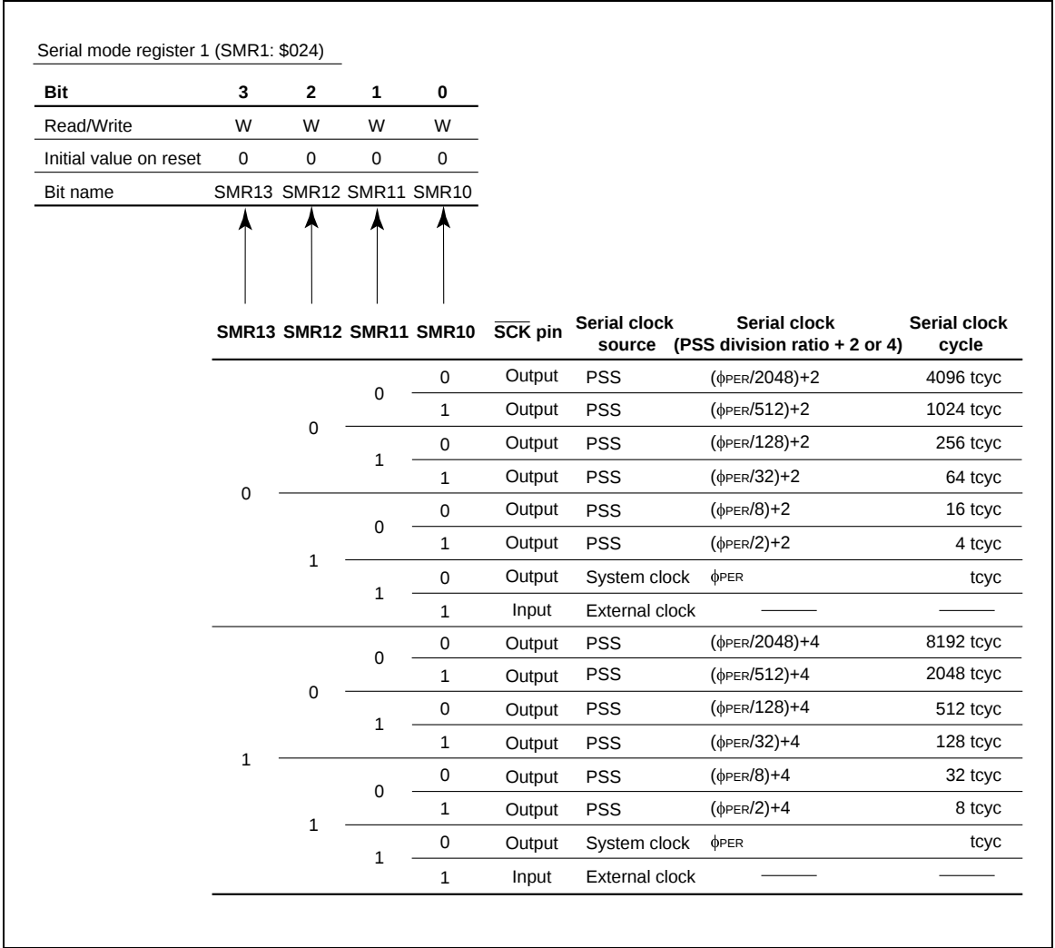
Figure 56 Serial Mode Register 1 (SMR1)
