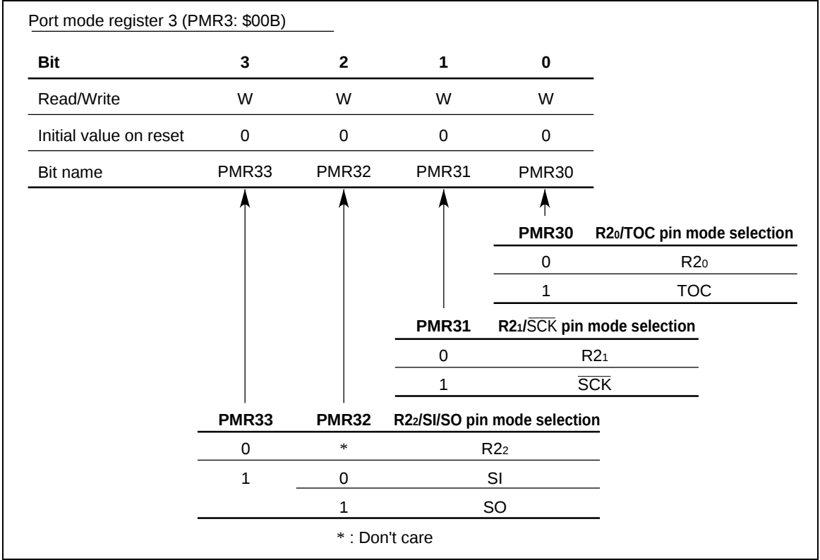
Figure 29 Port Mode Register 3 (PMR3: $00B)
