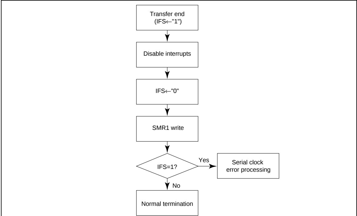
(1) Serial clock error detection flowchart
