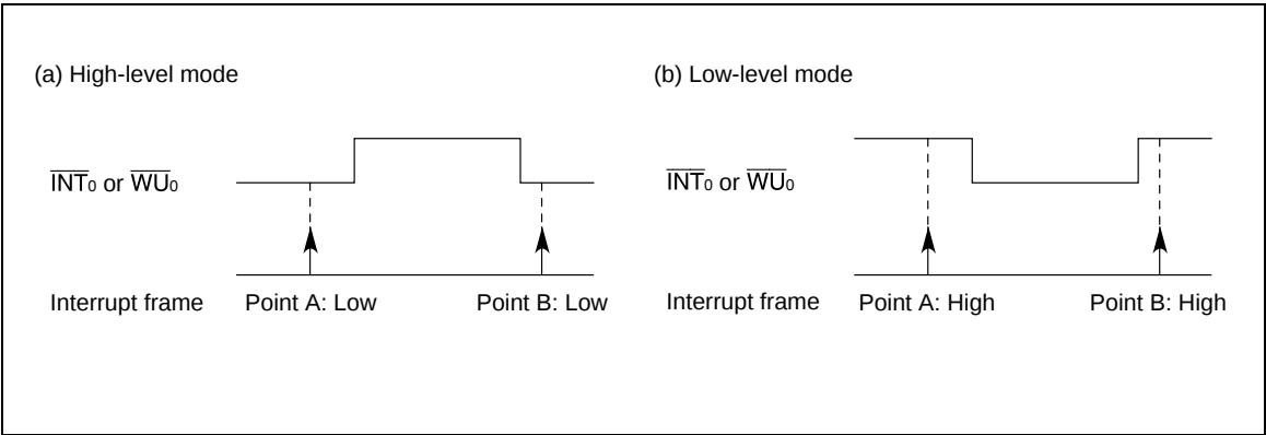
Figure 19 Sampling Examples
