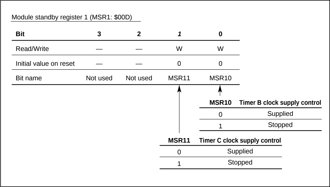
Figure 43 Module Standby Register 1 (MSR1)
