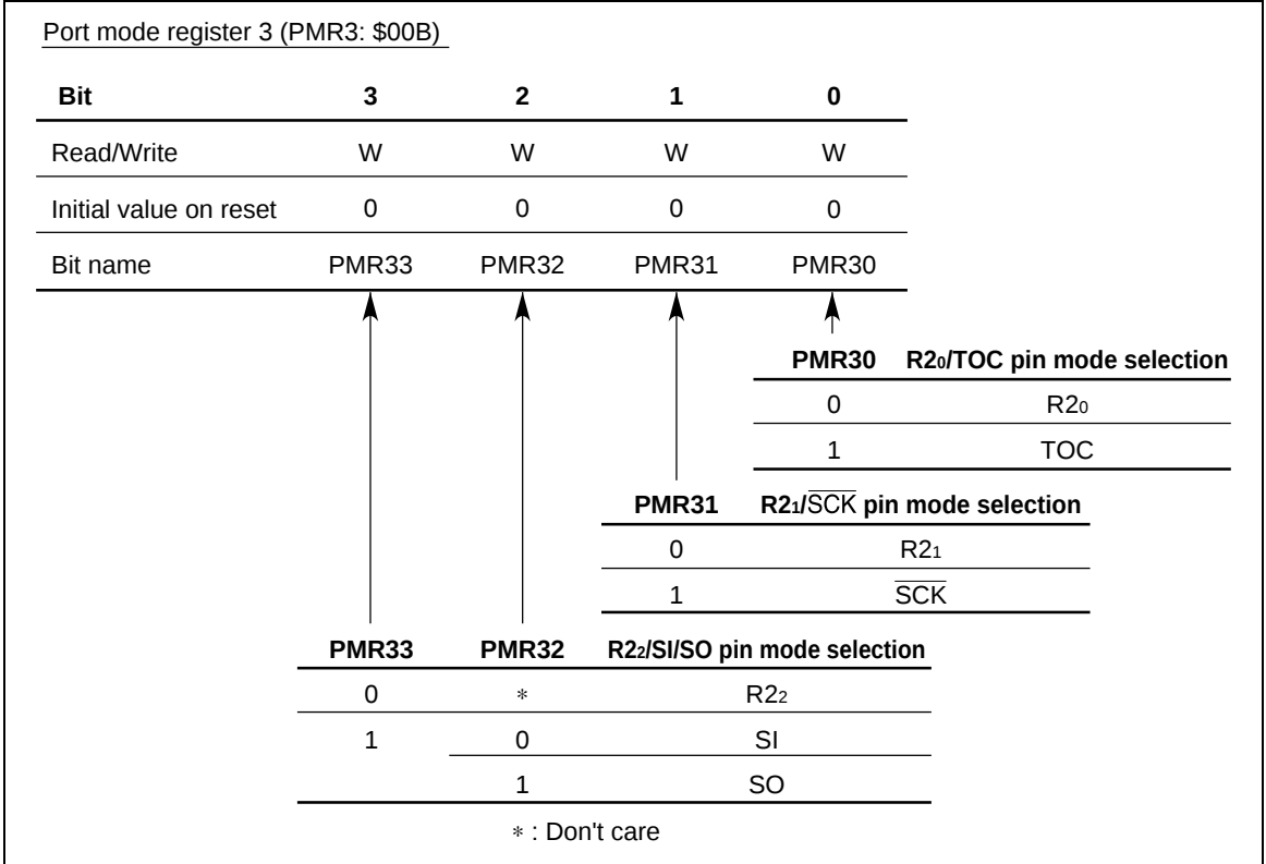
Figure 51 Port Mode Register 3 (PMR3)
