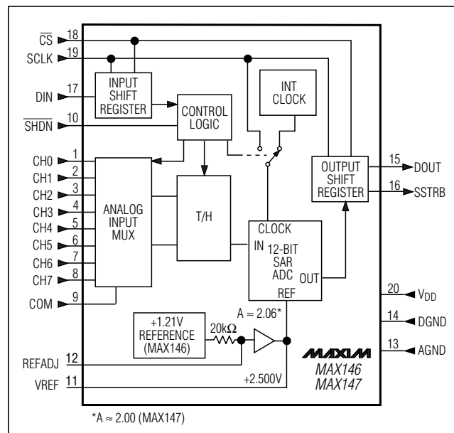
Figure 3. Block Diagram
