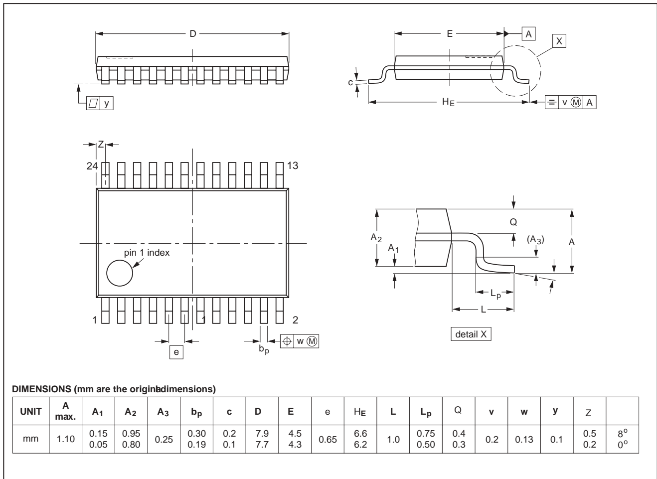
Figure 22: TSSOP24
