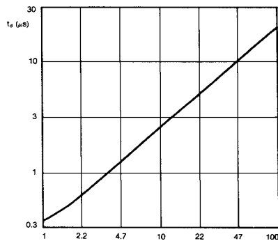
Figure 6. Oscillator Dead Time &amp; Frequency
