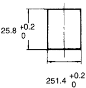
Mounting holes
