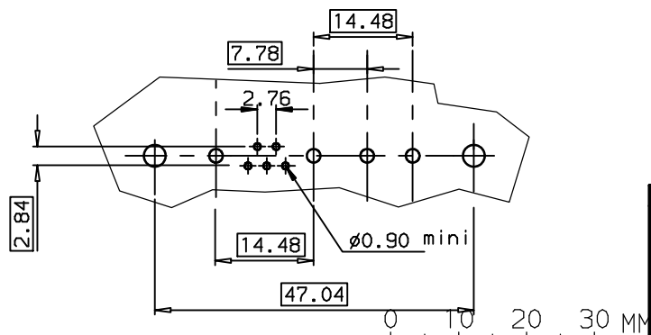
LAYOUT DIMENSIONS (after plating)
