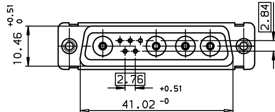
LAYOUT DIMENSIONS (after plating)
