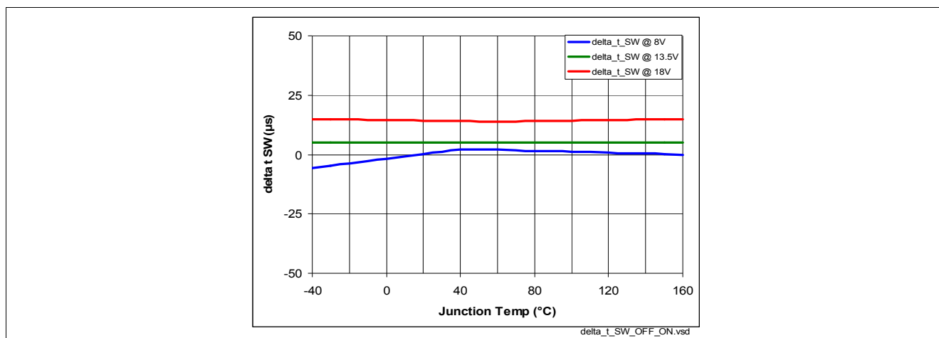
Figure 40 Turn ON / OFF matching \Delta t_{SW} = f(T_J; V_S) , R_L = 4 \Omega
