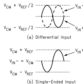
Figure 36. Expected Input Signal Range
