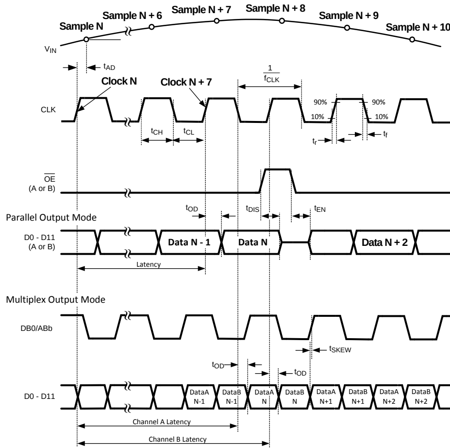
Figure 3. Output Timing
