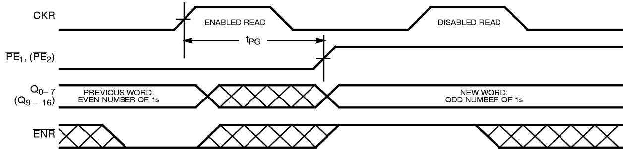
Even Parity Generation Timing Diagram [37, 38]
