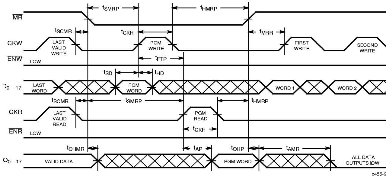
Master Reset (Programming Mode with Free-Running Clocks) Timing Diagram [19, 20]
