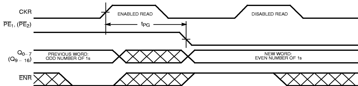
Even Parity Generation Timing Diagram [37, 39]
