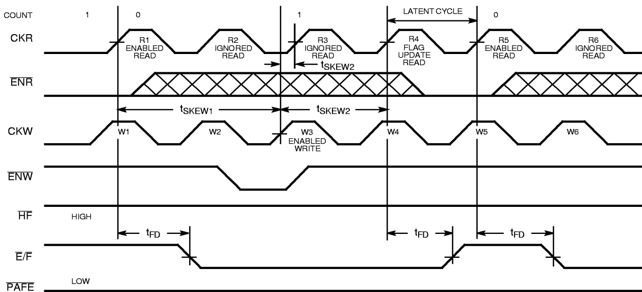
Read to Empty Timing Diagram with Free-Running Clocks [21, 22, 23, 24]
