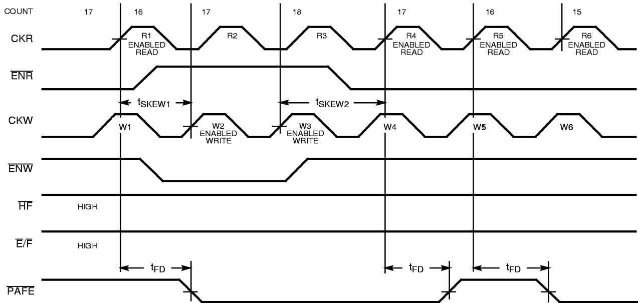
Read to Almost Empty Timing Diagram with Free-Running Clocks [21, 24, 26]
