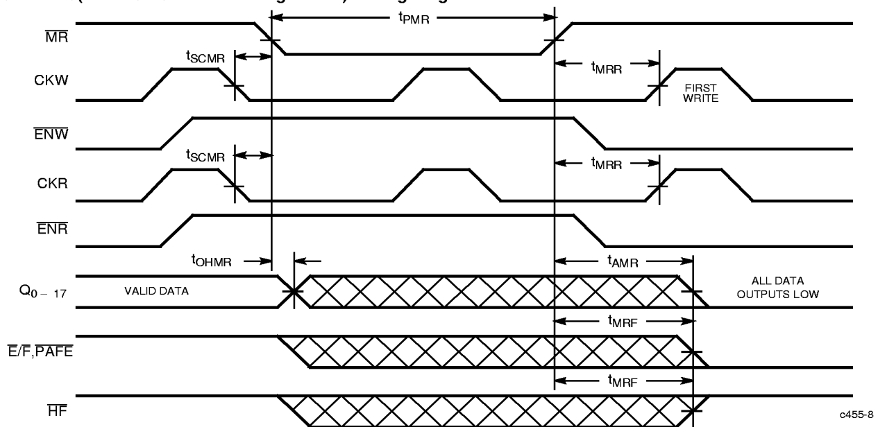
Master Reset (Default with Free-Running Clocks) Timing Diagram [17, 18, 19, 20]
