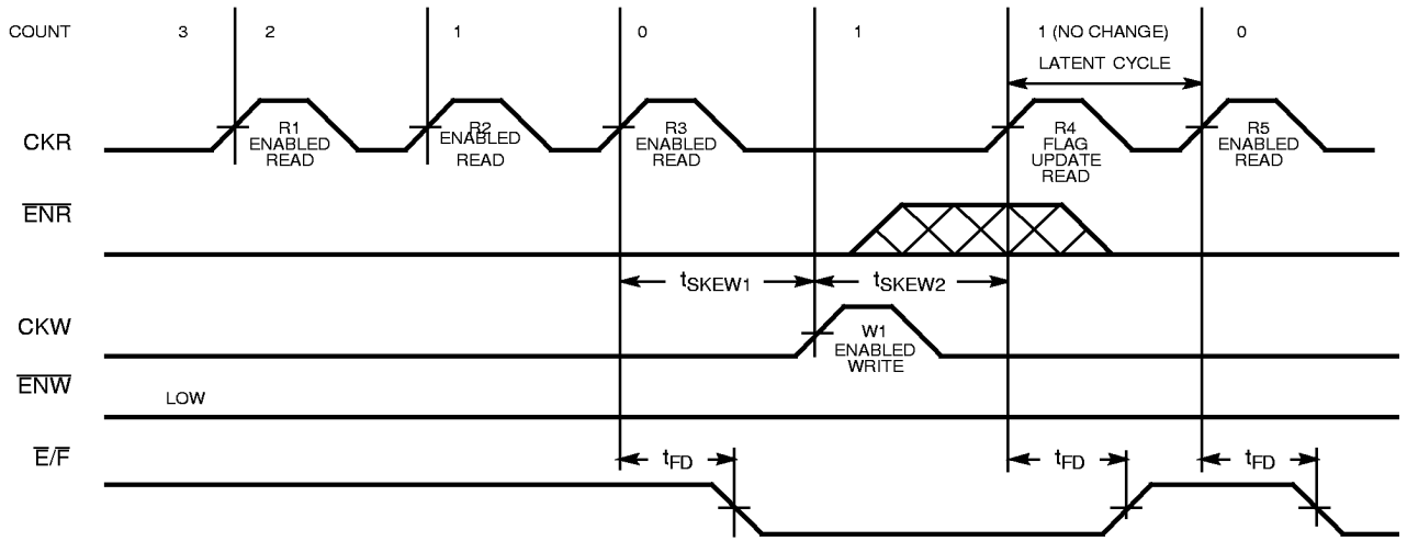
Read to Empty Timing Diagram [21, 24, 25]
