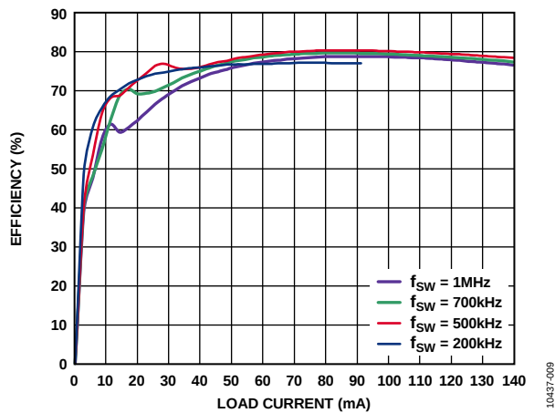
Figure 11. 5 V In to 15 V Out Efficiency at Various Switching Frequencies with 1:3 Coilcraft Transformer (JA4650-BL)
