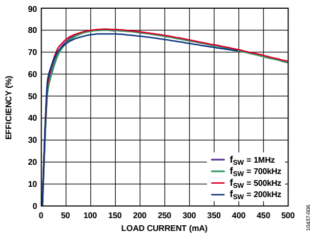
Figure 6. Typical Efficiency at 5 V In to 5 V Out at Various Switching Frequencies with 1:2 Halo Transformer (TGSAD-260V6LF)
