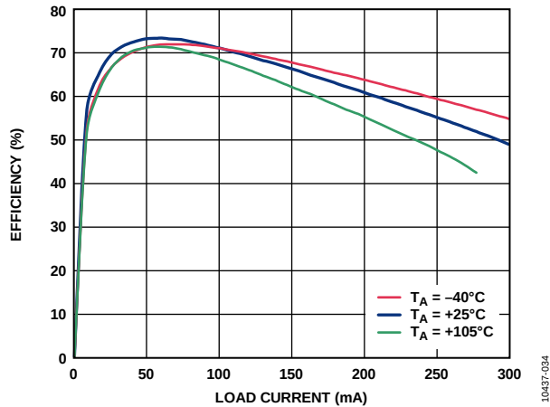
Figure 10. Typical Efficiency at 3.3 V In to 5 V Out over Temperature with 1:3 Halo Transformer (TGSAD-290V6LF) at 500 kHz f_{sw}
