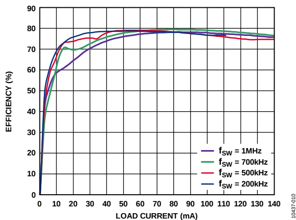
Figure 12. 5 V In to 15 V Out Efficiency at Various Switching Frequencies with 1:3 Halo Transformer (TGSAD-290V6LF)
