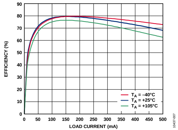
Figure 7. 5 V In to 5 V Out Efficiency over Temperature with 1:2 Coilcraft Transformer (JA4631-BL) at 500 kHz f_{SW}
