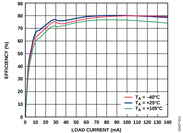
Figure 13. 5 V In to 15 V Out Efficiency over Temperature with 1:3 Coilcraft Transformer (JA4650-BL) at 500 kHz f_{sw}
