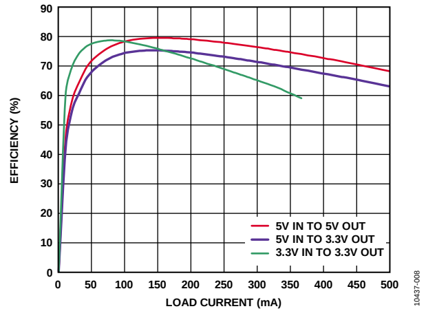
Figure 8. Single-Supply Efficiency with 1:2 Coilcraft Transformer (JA4631-BL) at 500 kHz f_{SW}
