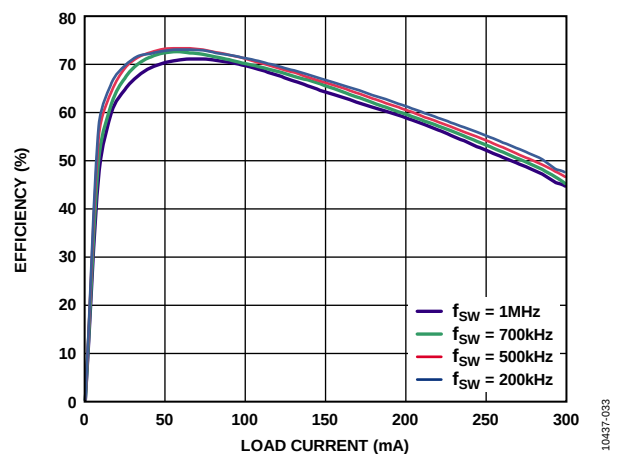
Figure 9. Typical Efficiency at 3.3 V In to 5 V Out at Various Switching Frequencies with 1:3 Halo Transformer (TGSAD-290V6LF)
