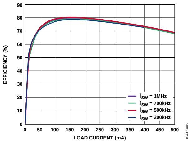
Figure 5. Typical Efficiency at 5 V In to 5 V Out at Various Switching Frequencies with 1:2 Coilcraft Transformer (JA4631-BL)
