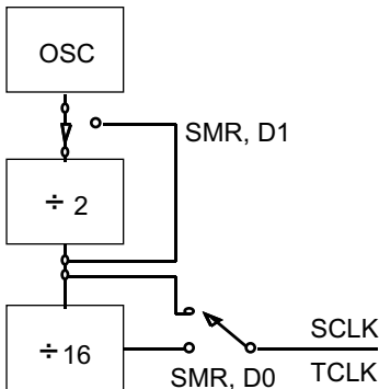
Figure 36. SCLK Circuit
