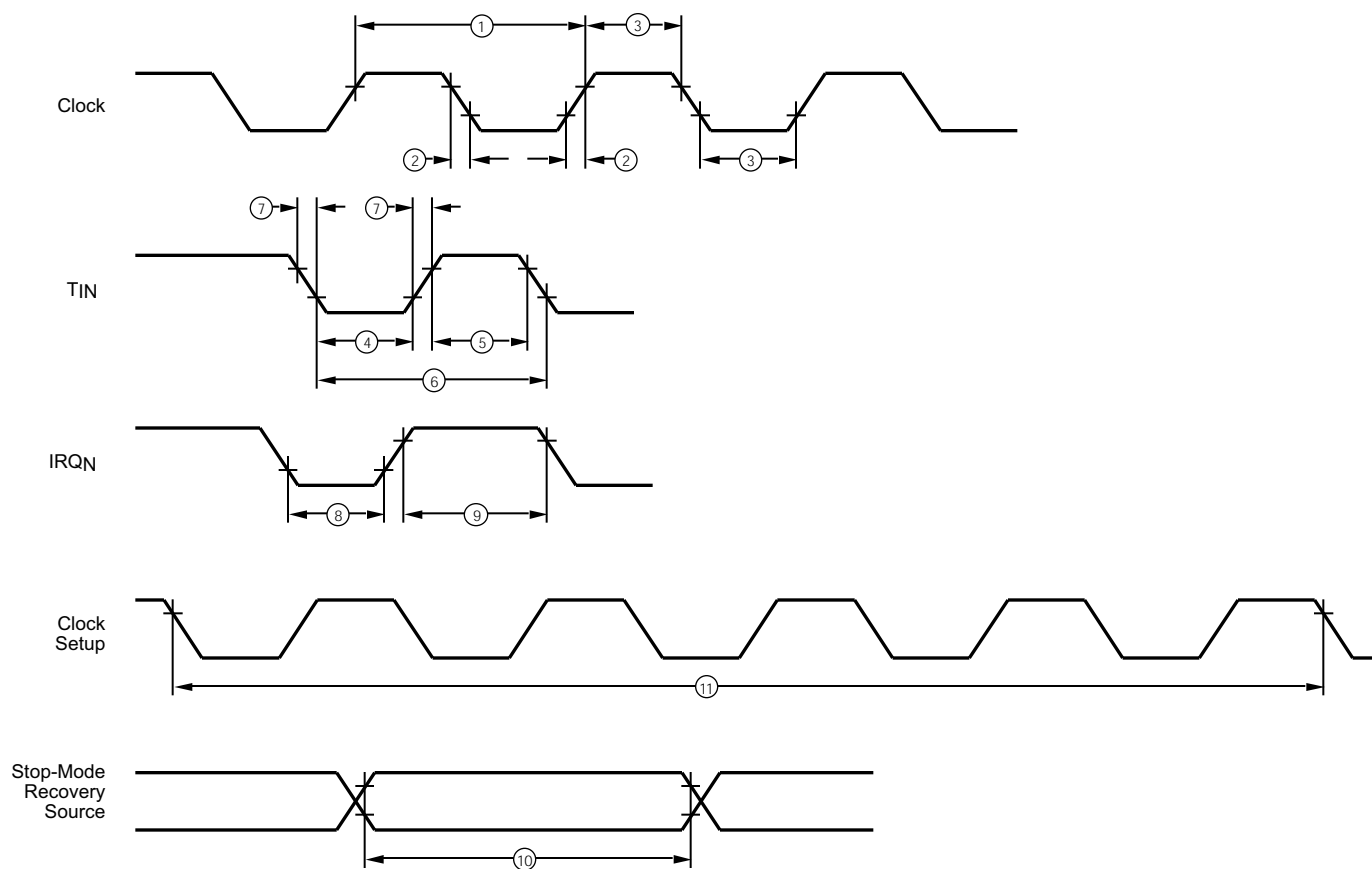
Figure 9. Additional Timing
