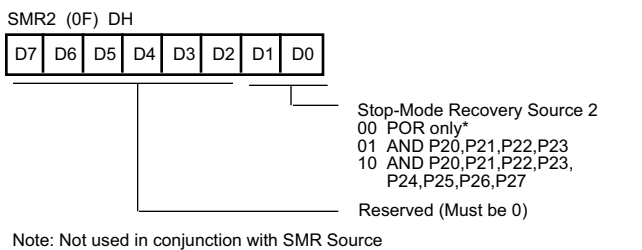
Figure 35. Stop-Mode Recovery Register 2 ([0F] DH: Write-Only)
