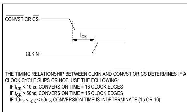
Figure 10. Clock and Control Synchronization
