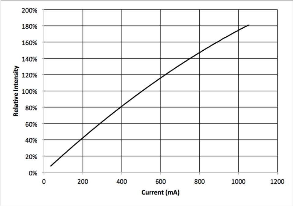
Figure 2: Typical Flux vs. Drive Current, Tj = 25°C
