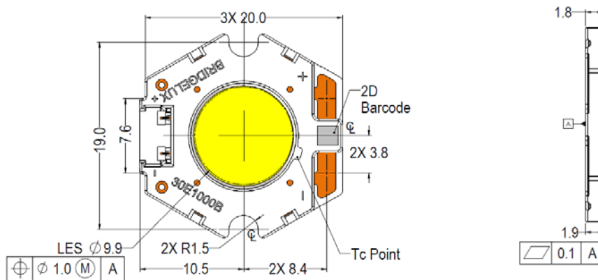
Figure 9: Drawing for Vero 10 LED Array
