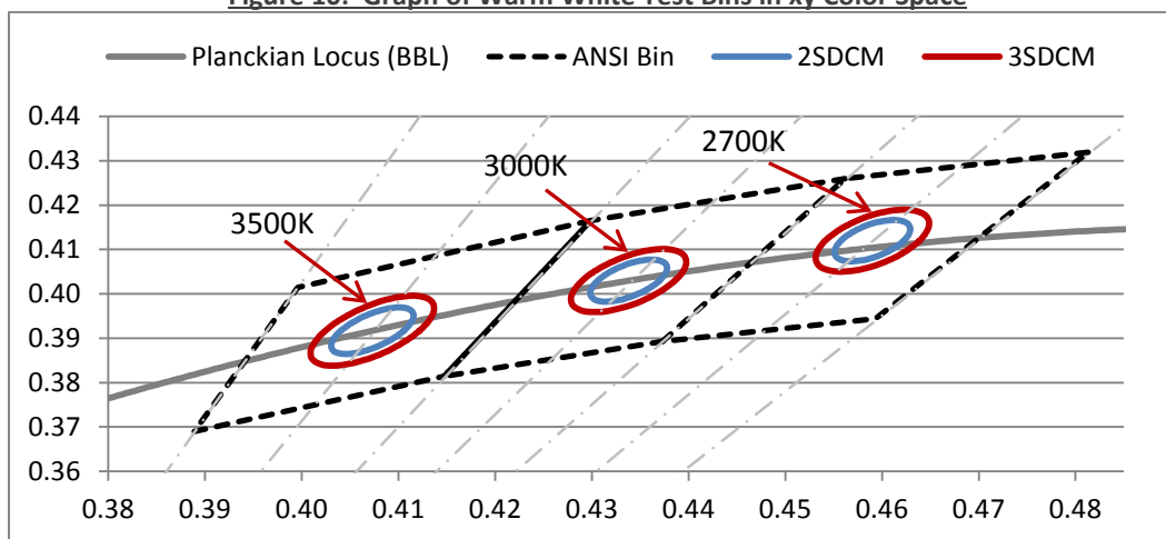
Figure 10: Graph of Warm White Test Bins in xy Color Space
