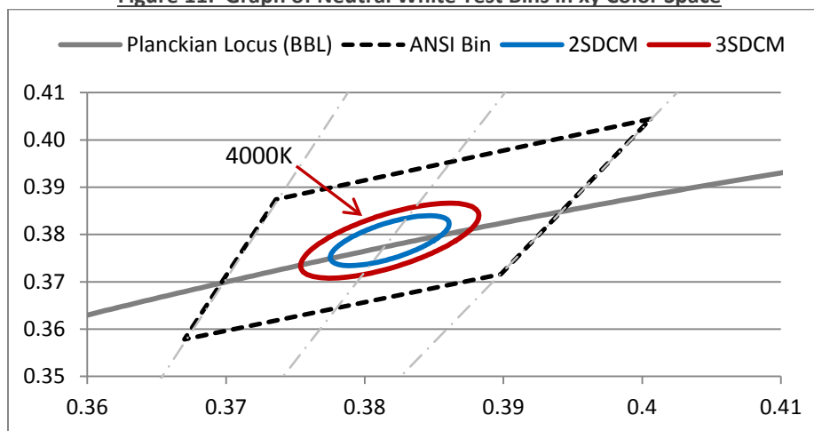
Figure 11: Graph of Neutral White Test Bins in xy Color Space
