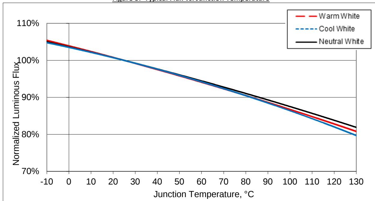
Figure 3: Typical Flux vs. Junction Temperature
