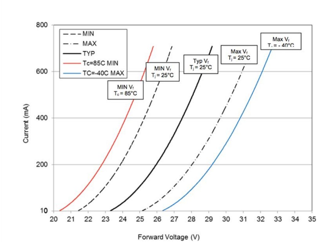
Figure 1: Drive Current vs. Forward Voltage
