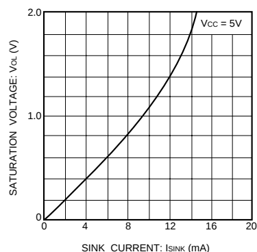
Fig. 3 Output voltage (logic 0 side) characteristics
