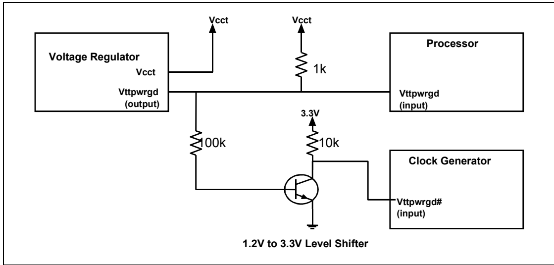
Figure 3. VTTPWRGD System-Level Connections
