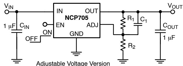
Figure 1. Typical Application Schematics
