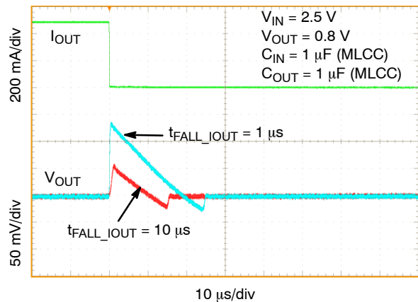
Figure 55. Load Transient Response – Falling Edge, V_{OUT} = 0.8\text{ V} , I_{OUT} = 1\text{ mA} to 500\text{ mA} , t_{FALL\_IOUT} = 1\text{ μs} , 10\text{ μs}
