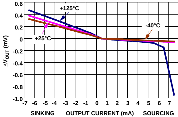
FIGURE 33. LOAD REGULATION OVER TEMPERATURE
