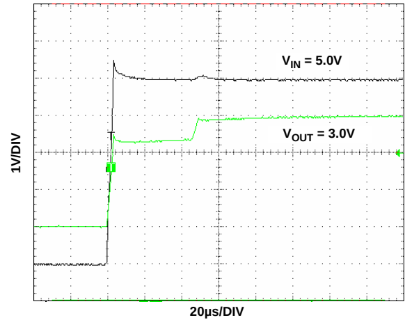
FIGURE 51. TURN-ON TIME
