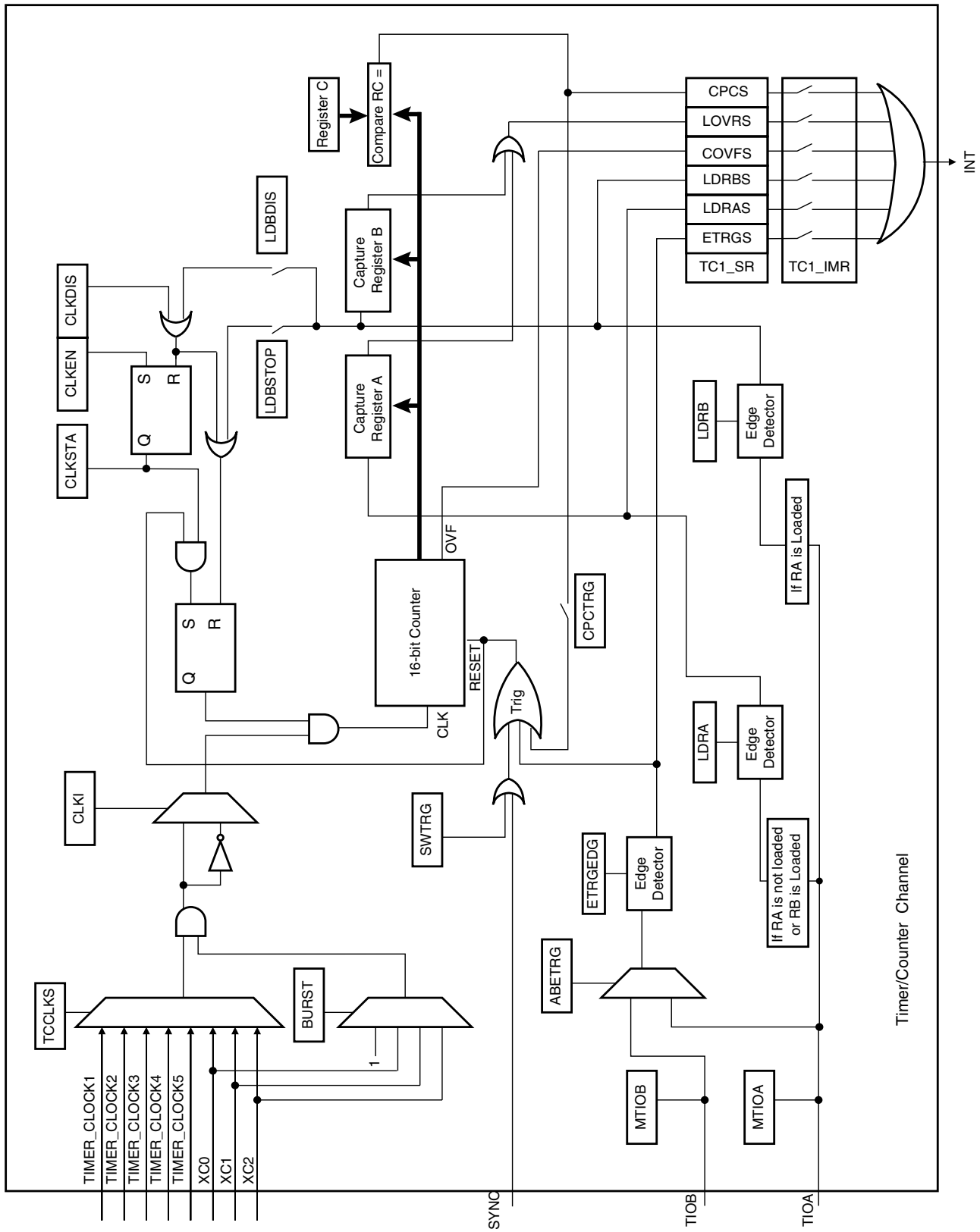
Figure 31-4. Capture Mode
