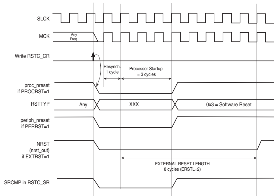
Figure 13-7. Software Reset
