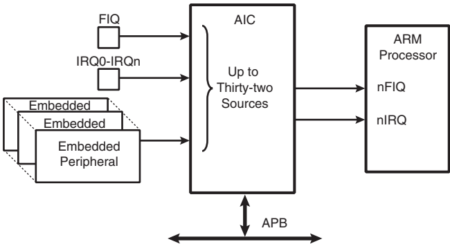
Figure 22-1. Block Diagram
