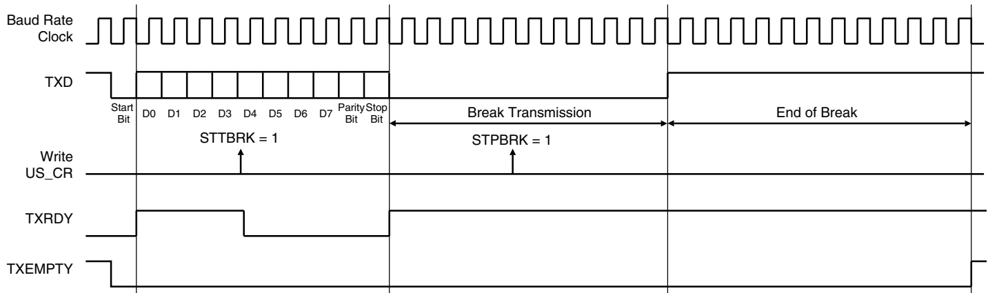
Figure 29-26. Break Transmission
