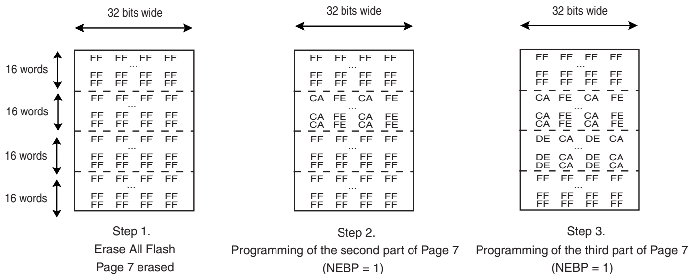
Figure 19-6. Example of Partial Page Programming:
