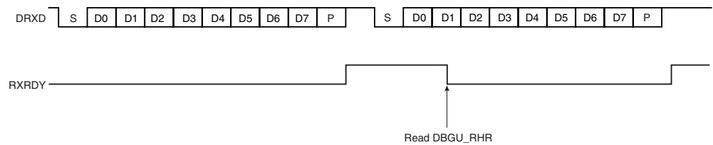
Figure 25-6. Receiver Ready
