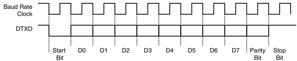
Figure 25-10. Character Transmission
