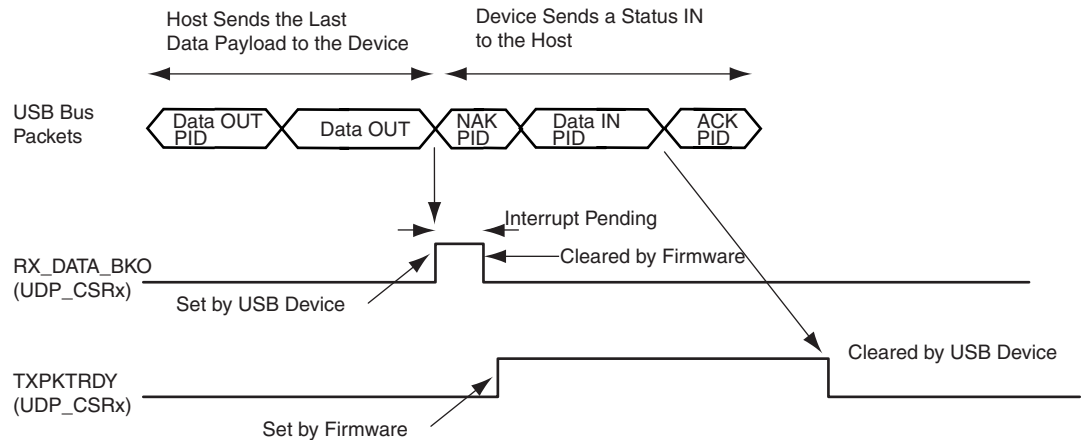
Figure 33-12. Data Out Followed by Status IN Transfer.
