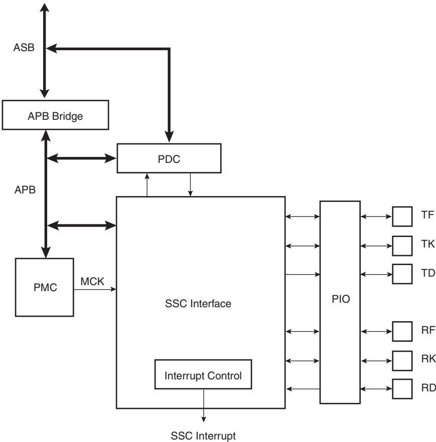
Figure 30-1. Block Diagram
