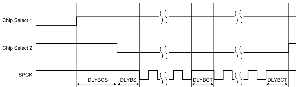
Figure 27-7. Programmable Delays
